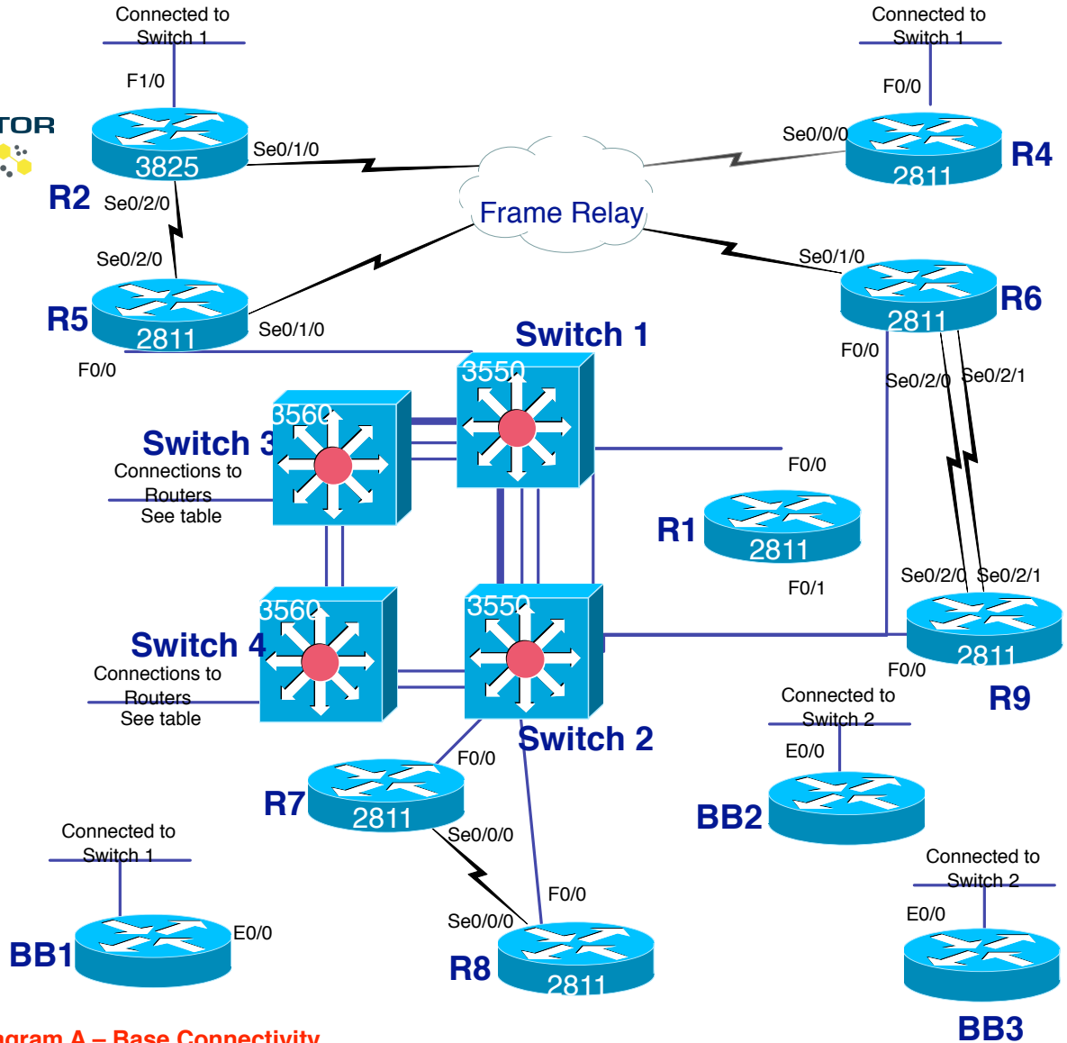
Diagram A – Base Connectivity
